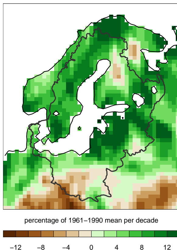
Figure 3.2: Trends in winter (DJF) precipitation totals 1973-2002 in units of relative change compared to the 1961-1990 mean precipitation (according to the CRU TS 2.1 data), negative trends are marked by thin solid contours.
